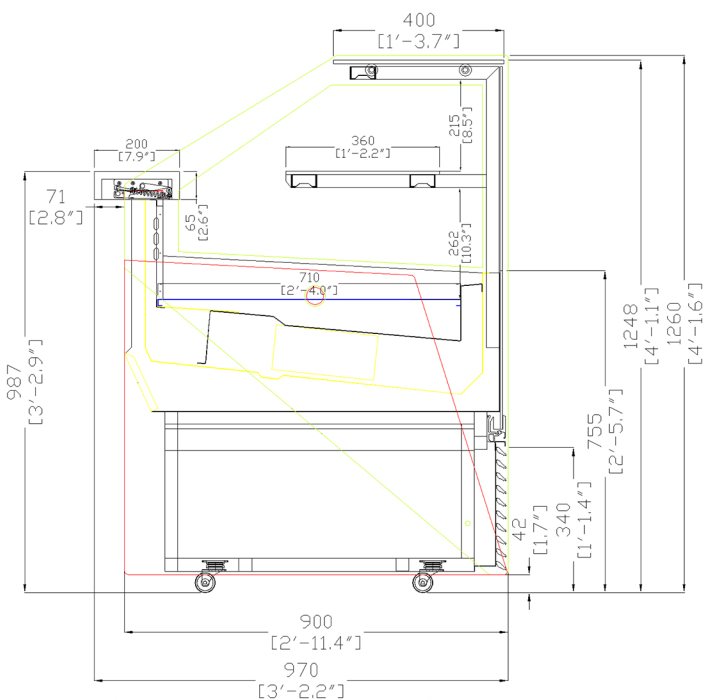
SIDE VIEW (Wireframe) Rear counter CLOSE position
