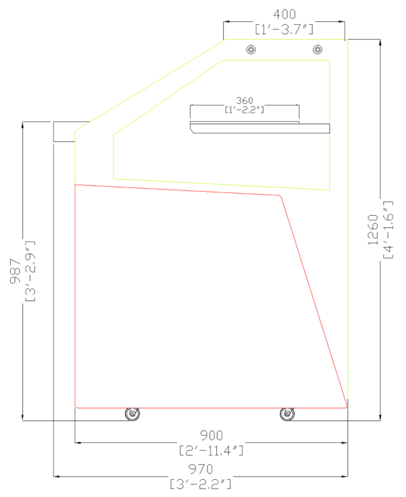
SIDE VIEW (Hide) Rear counter CLOSE position
